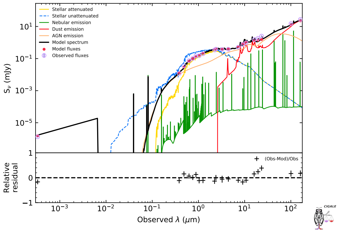
Fig. 3. An example SED generated by the pcigale-plots command.
