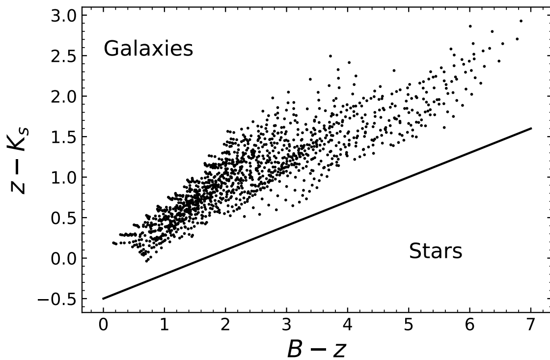
Fig. 4. A BzK diagram simulated in the savefluxes mode. The solid line indicates the empirical separation between galaxies and stars (Daddi et al., 2004).
